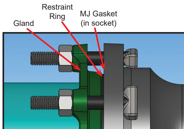
View when installed on ductile iron or C900
