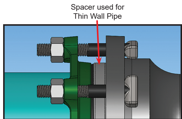
View when installed on thin walled PVC or PVCO
