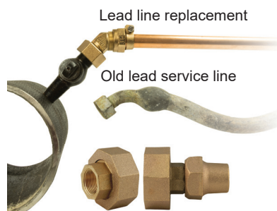
Lead Flanged / Wiped Lead Conversion Connections (Conversion of Lead Service Corp Stops) Catalog Section A
