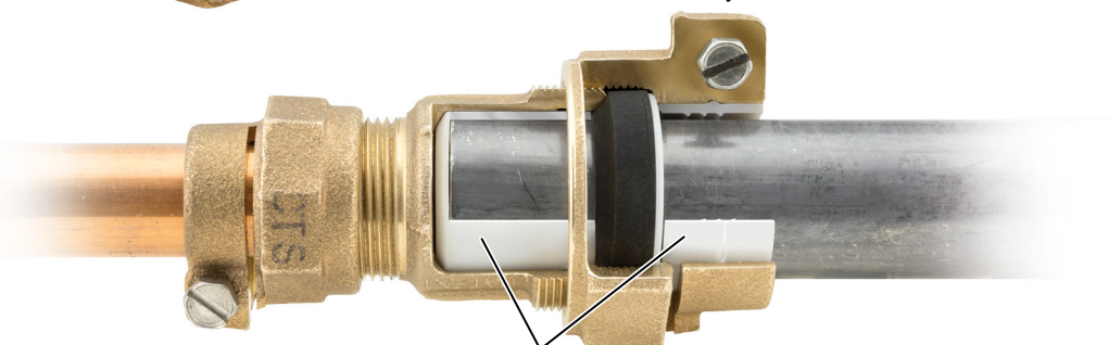
Cut-away View
