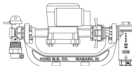
Example of a complete Yoke meter setting using a 500 Series Yoke Bar, an Angle Ball Inlet Valve, a standard Expansion Connection and an Angle Cartridge Dual Check Outlet Valve.
