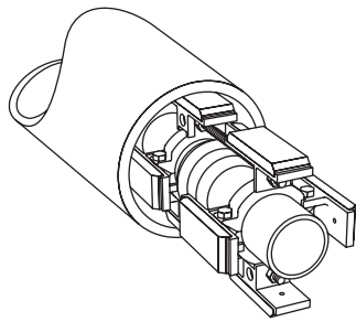
4", 6" and 8" Restrained Casing Spacer for Pipe Bell Joint
