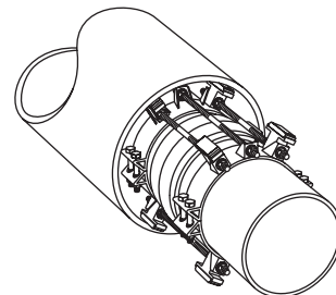
14" through 24" Restrained Casing Spacer for Pipe Bell Joint
