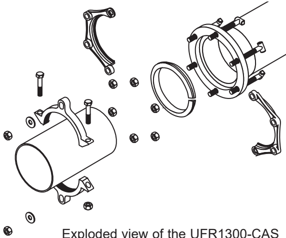
Exploded view of the UFR1300-CAS
