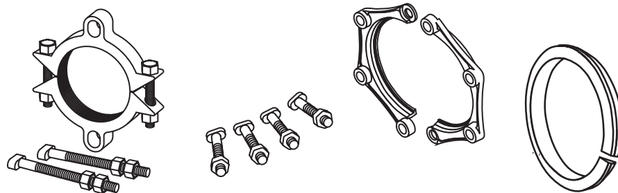
Exploded view of the UFR1300-CAS
