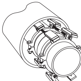
10" and 12" Restrained Casing Spacer for Pipe Bell Joint
