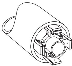
4", 6" and 8" Casing Spacer for support of pipe
