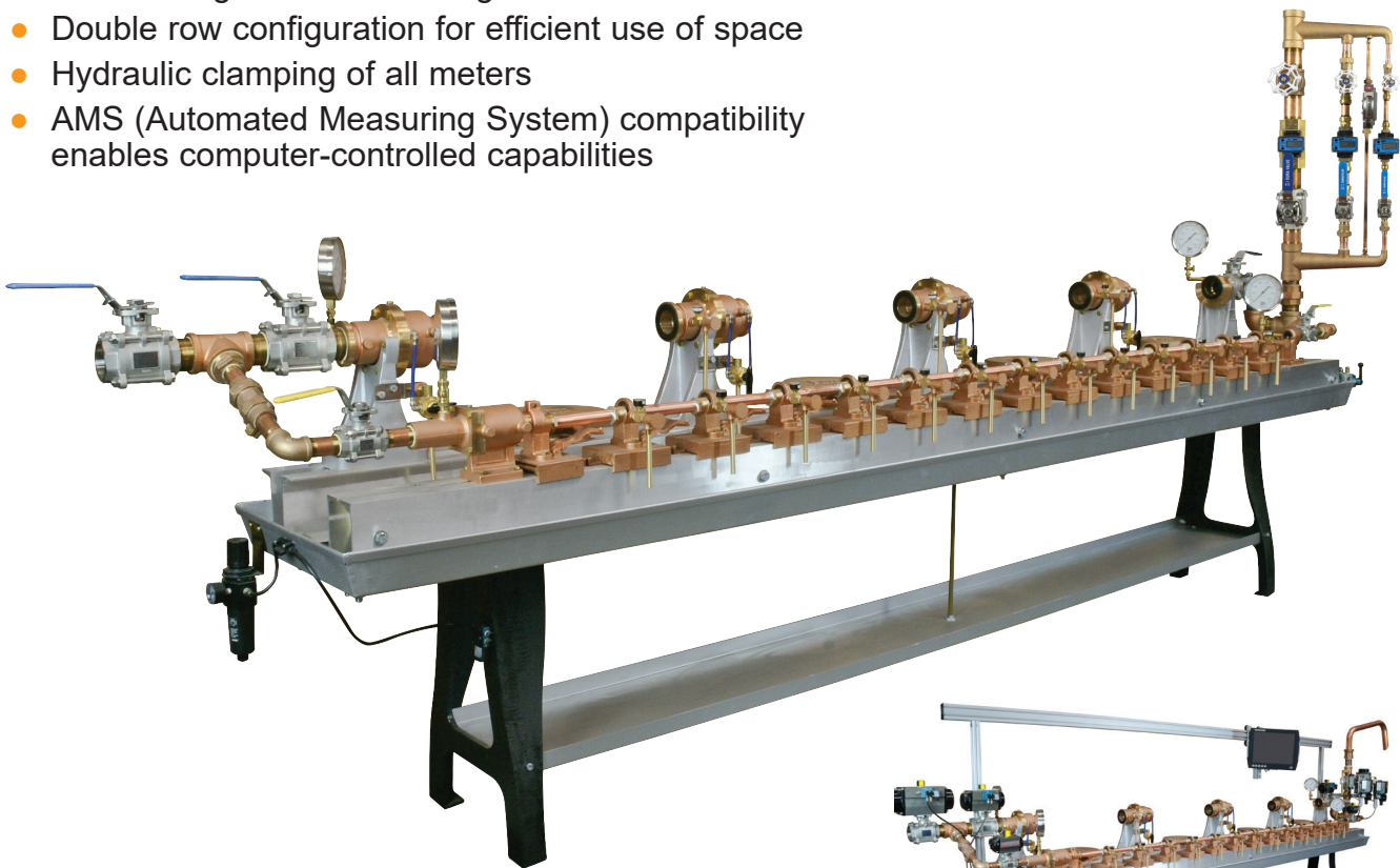
Combo test bench with AMS option
