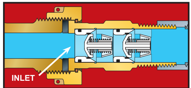
Negative inlet water pressure - check valves close
