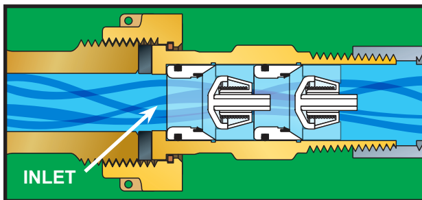
Positive inlet water pressure - check valves open
