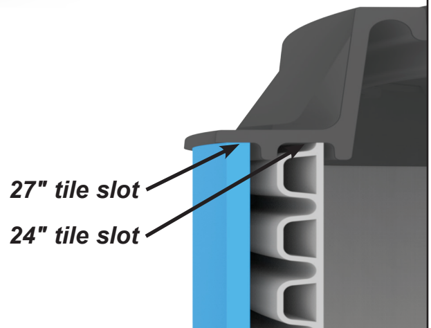
A656H - for 24" and 27" Tile
