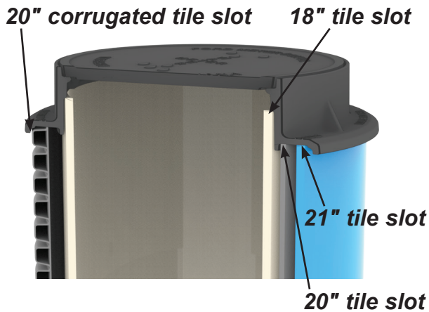
A6234H - for 18", 20", and 21" Tile
