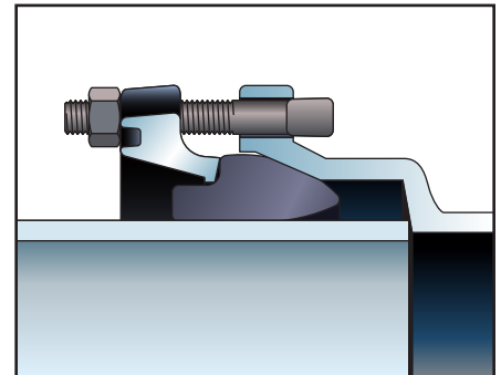
14"-24" Transition Gasket 24" Metric-Seal Gasket
