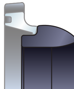
14"-24" Transition Gasket 24" Metric-Seal Gasket
