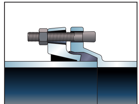
14"-20" Metric-Seal Gasket
