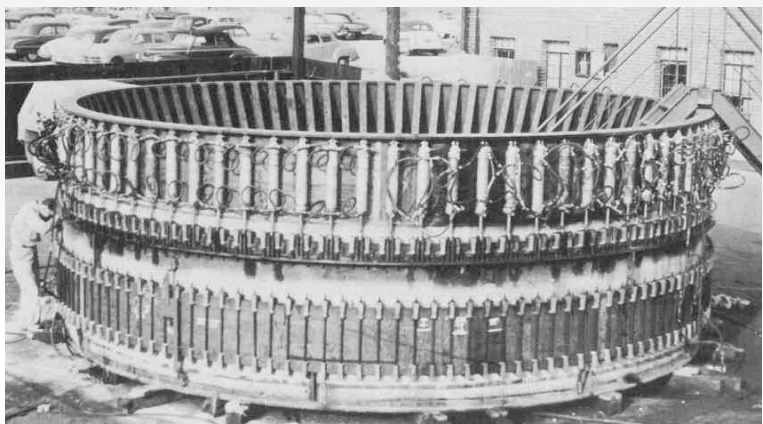
24 Foot Diameter Coupling for use in Garrison Dam, North Dakota
