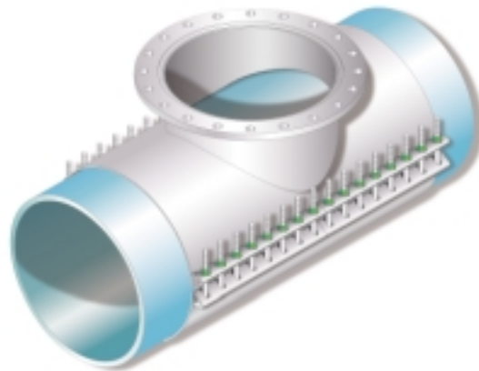
24" x 24" Ford FTSAS All Stainless Steel Tapping Sleeve
