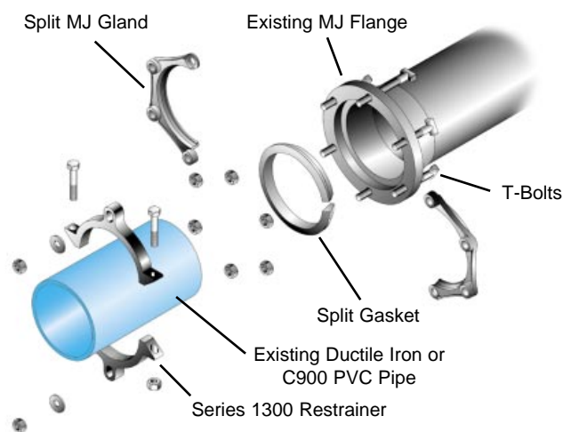
Exploded view of the UFR1300-CAS
