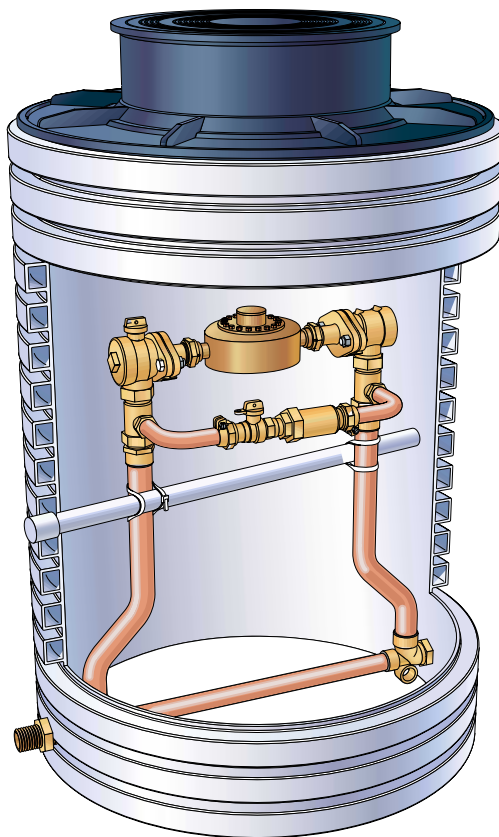
A 2" Plastic Pit Setter fitted with two A47 meter adapters change a 2" flanged meter setting to accommodate a 1" meter
