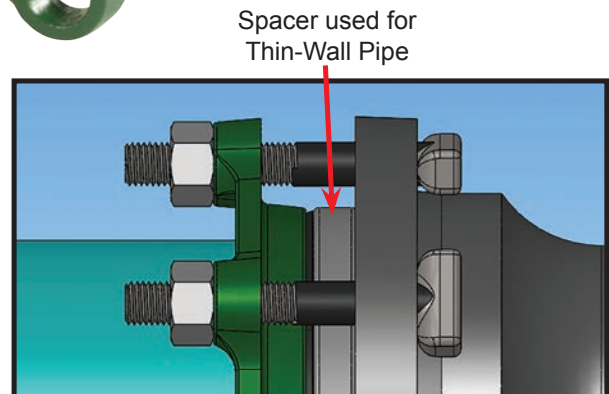
View when installed on thin-walled PVC or PVCO
