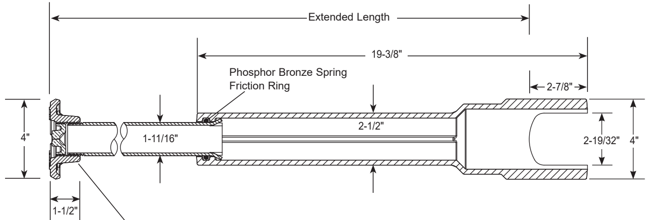
Type PL Lid - Plug style lid with 27/32" pentagon bolt
