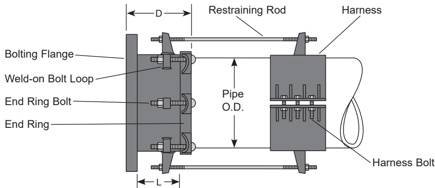
FCA Coupling with Restrainer Lug and Harness Assembly
