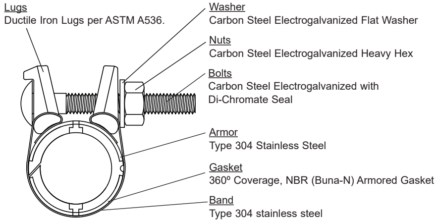
Dual Armor Design
