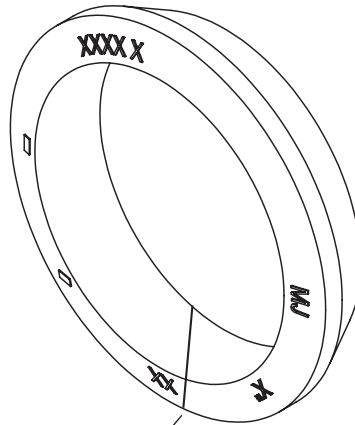
Split mechanical joint gasket AWWA C111
