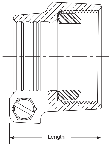
Pack Joint Nut Assembly for CTS
