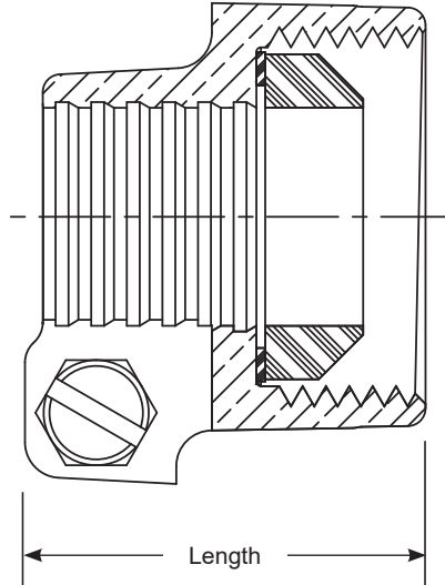
Pack Joint Nut Assembly for CTS
