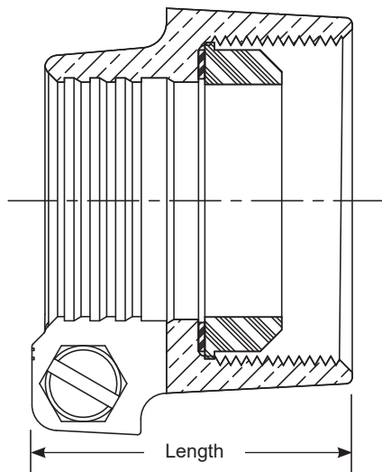
Pack Joint Nut Assembly for CTS
