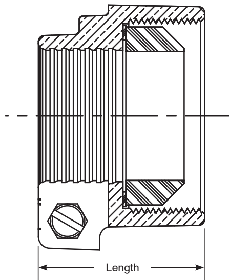
Pack Joint Nut Assembly
