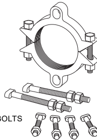
MECHANICAL JOINT GLAND AWWA C111
