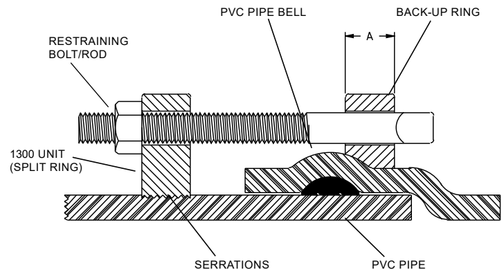
1350 Assembly
