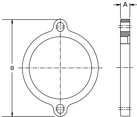
1350 Back-Up Ring
