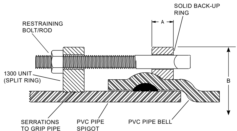
1350 Assembly
