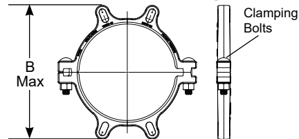
1360 Back-Up Ring
