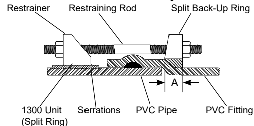
1360 Back-Up Ring
