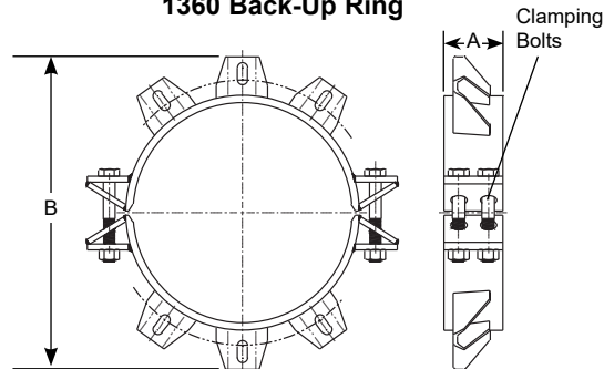
1360 Back-Up Ring
