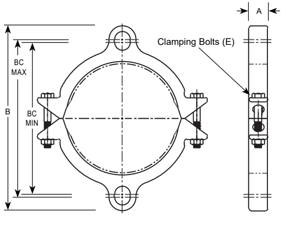
1360-P Back-Up Ring
