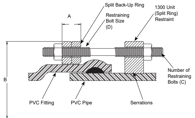
1360-P Assembly
