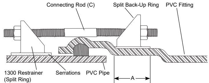
1360 Assembly
