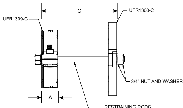
1369-C ASSEMBLY
