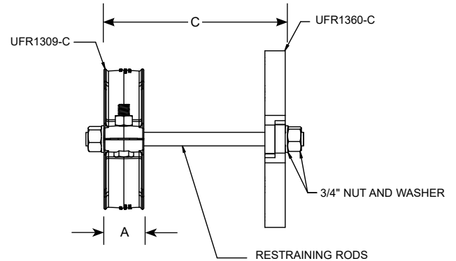
1369-C ASSEMBLY
