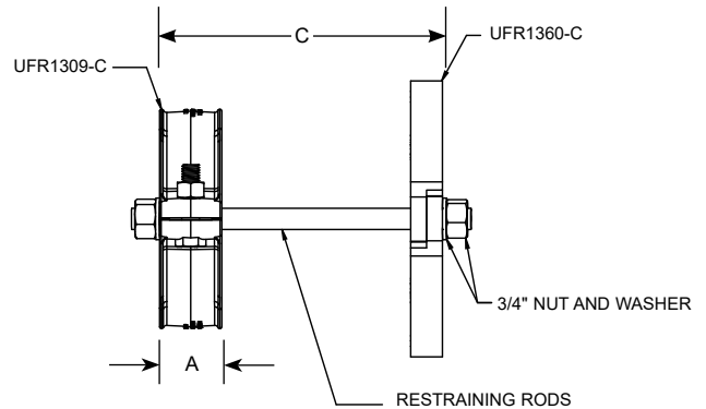
1369-C ASSEMBLY
