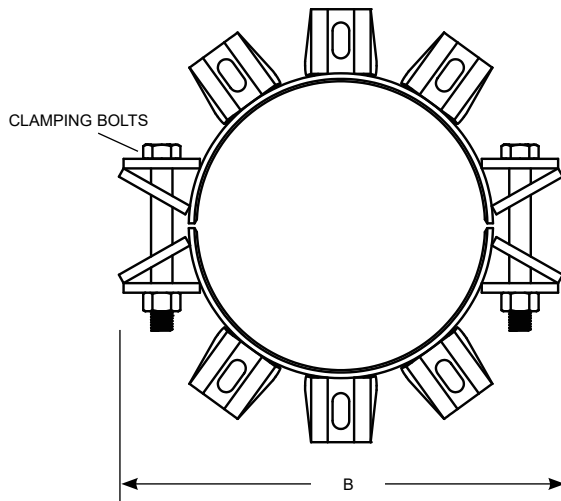
1309-C SPLIT RESTRAINT
