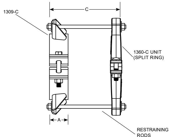
1369-C ASSEMBLY
