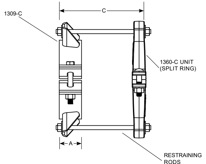
1369-C ASSEMBLY
