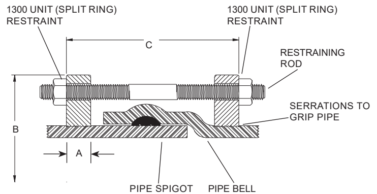
1390 ASSEMBLY
