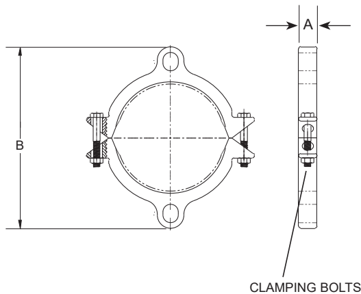
1300 SPLIT RESTRAINT
