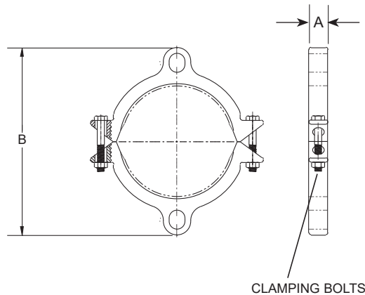
1300 SPLIT RESTRAINT
