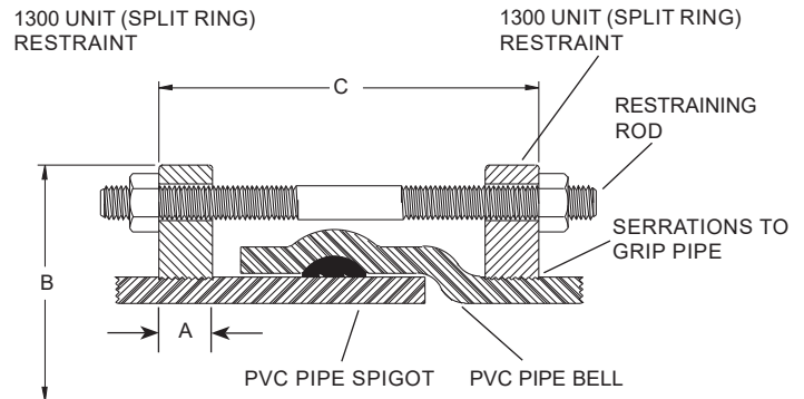
1390 ASSEMBLY
