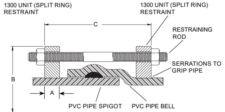
1390 ASSEMBLY
