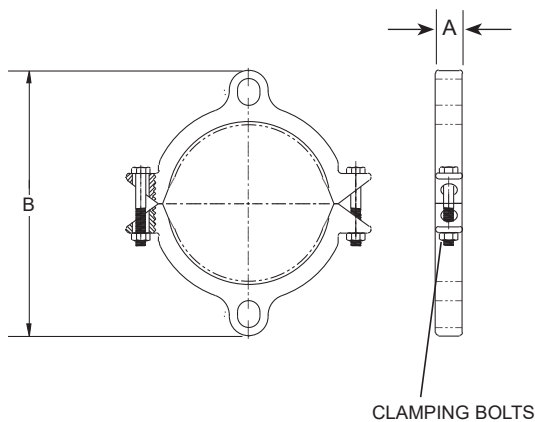
1300 SPLIT RESTRAINT
