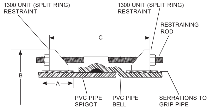
1390 ASSEMBLY
