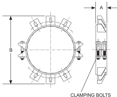
1300 SPLIT RESTRAINT
