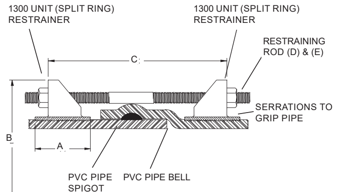
1390 ASSEMBLY
