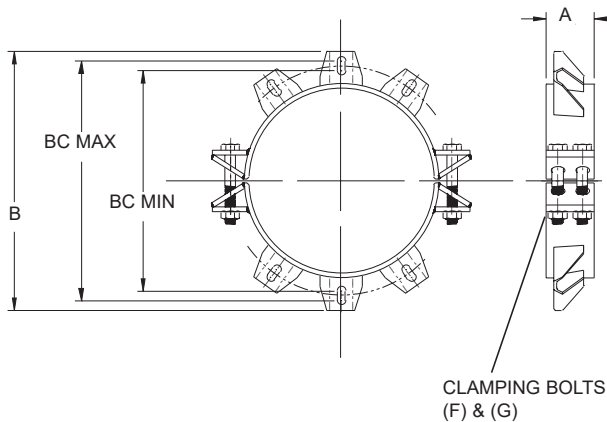
1300 SPLIT RESTRAINER
