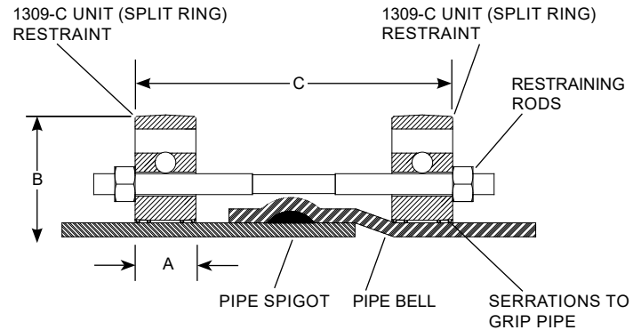
1399-C ASSEMBLY
