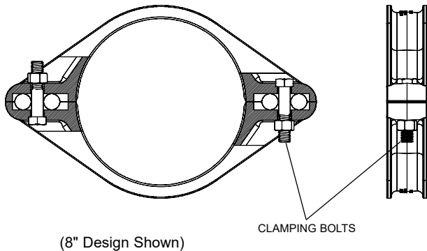
1309-C SPLIT RESTRAINT
