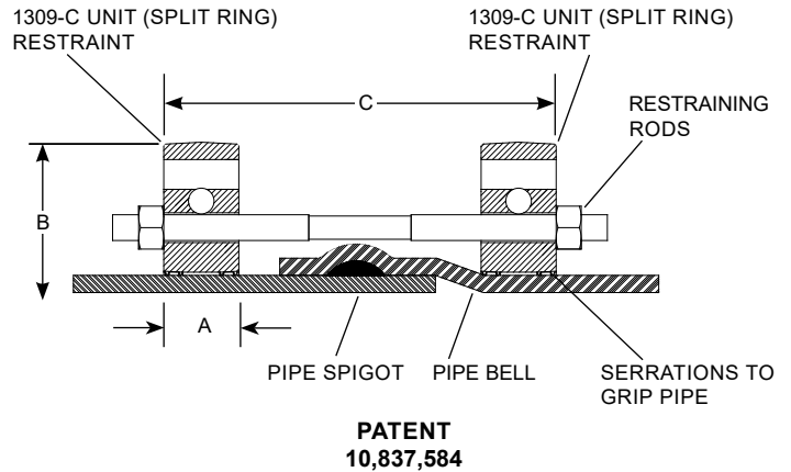
1399-C ASSEMBLY
