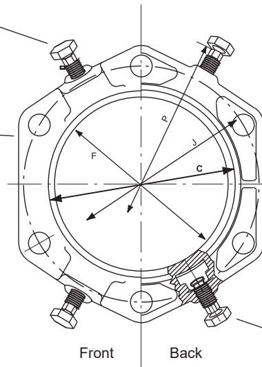
EPDM gasket AWWA C111
