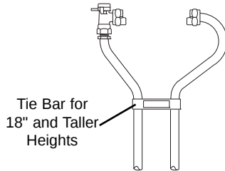
Male Threads for Pack Joint Assemblies (PJAx-1x-NL)
