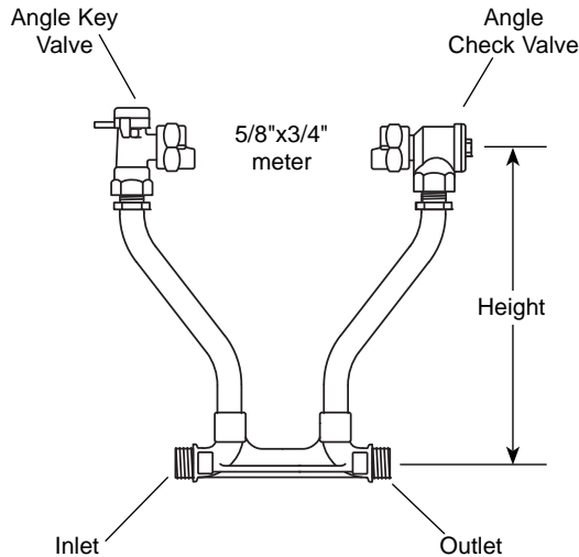
Male Threads for Pack Joint Assemblies (PJAx-1x-NL)
