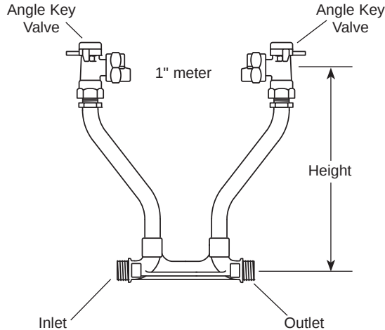
Male Threads for Pack Joint Assemblies (PJAx-4x-NL)
